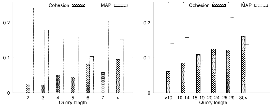
FIGURE 2: Cohesion scores and mean average precision (map), for title (left) and description queries (right), binned by query length (x-axis).
